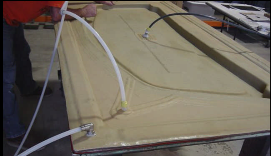
Resin Infusion – Complete * Note – no resin in vacuum waste line
