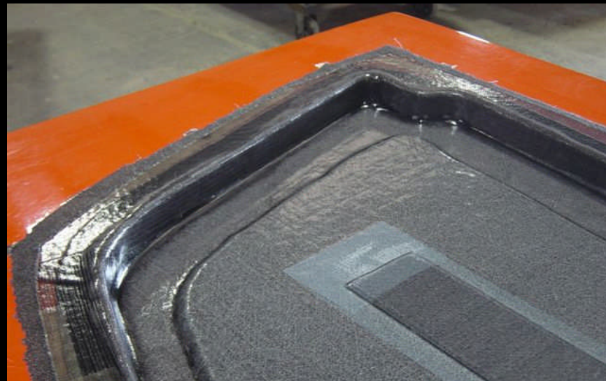
Even Wet Out Laminate – No Bridging
